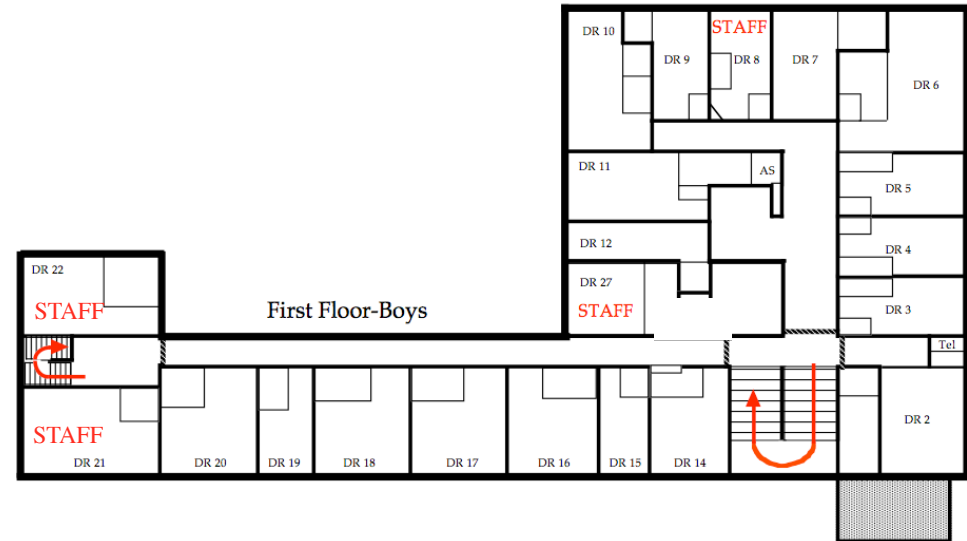
First Floor-Boys
